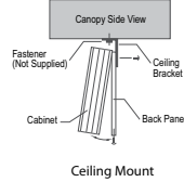
Ceiling Mount
