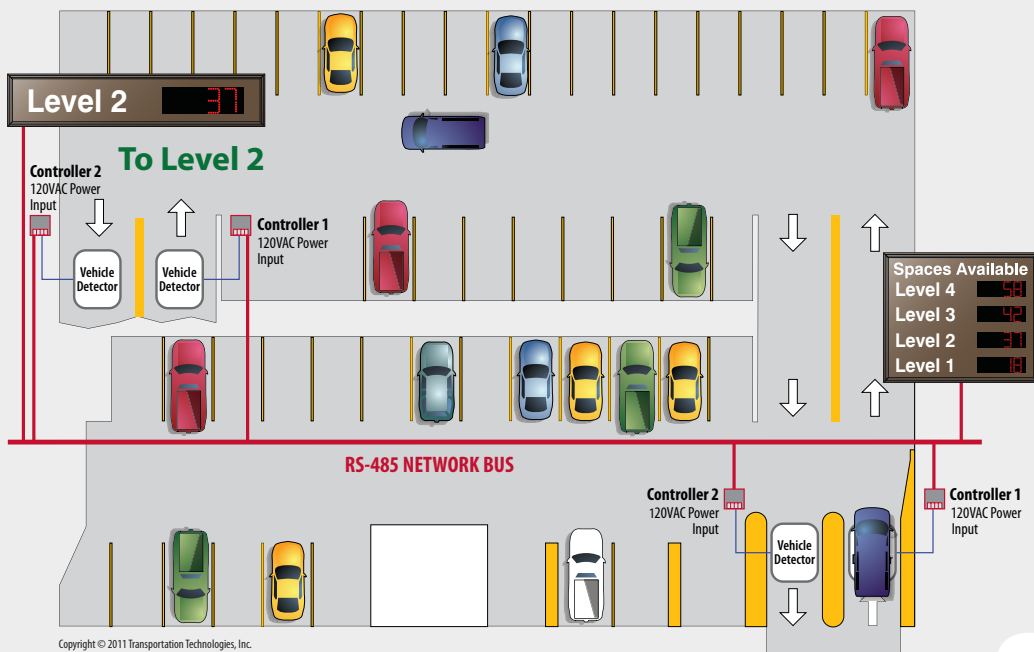
TYPICAL PARKING GARAGE LAYOUT
